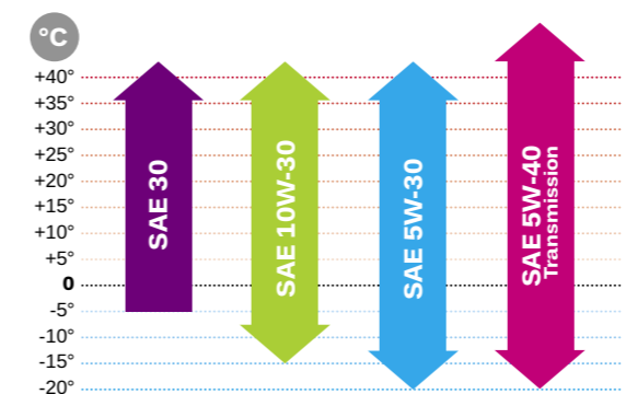
Temperature performance
