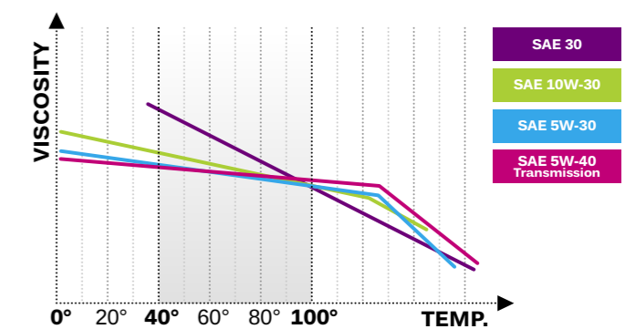
Viscosity performance
